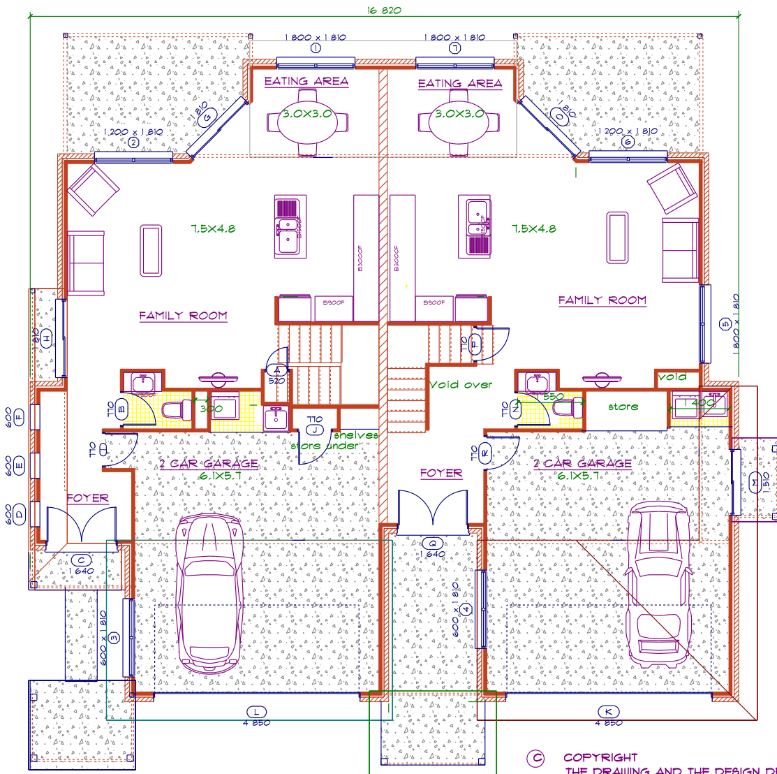
FLOOR PLAN
